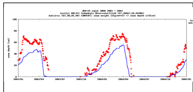
Figure 3. Temporal variation of snow depth by in-situ observation (red triangle) and by GLDAS-JRA25 experiment (blue line) from 2003 to 2004 at BALTEX Sodankyla, Finland (67.36667N, 26.62906E).
