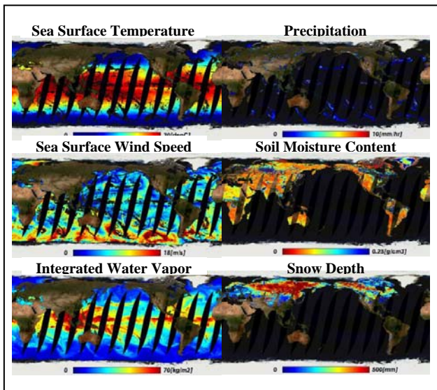
Figure 1. AMSR2 sample products in snap-shot (example produced by AMSR-E data).
