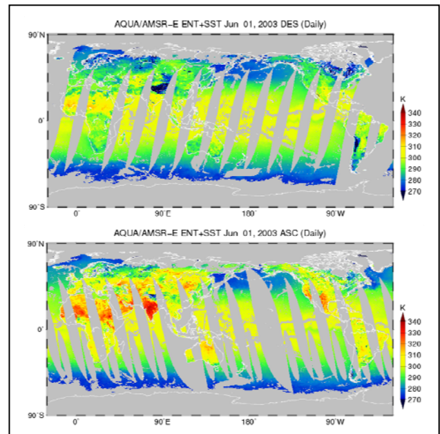
Figure 5. Example of ENT merged with SST, both retrieved from AMSR-E, for 1st June 2003 for descending (upper) and ascending (lower) orbits (Fujii et al. , 2010).
