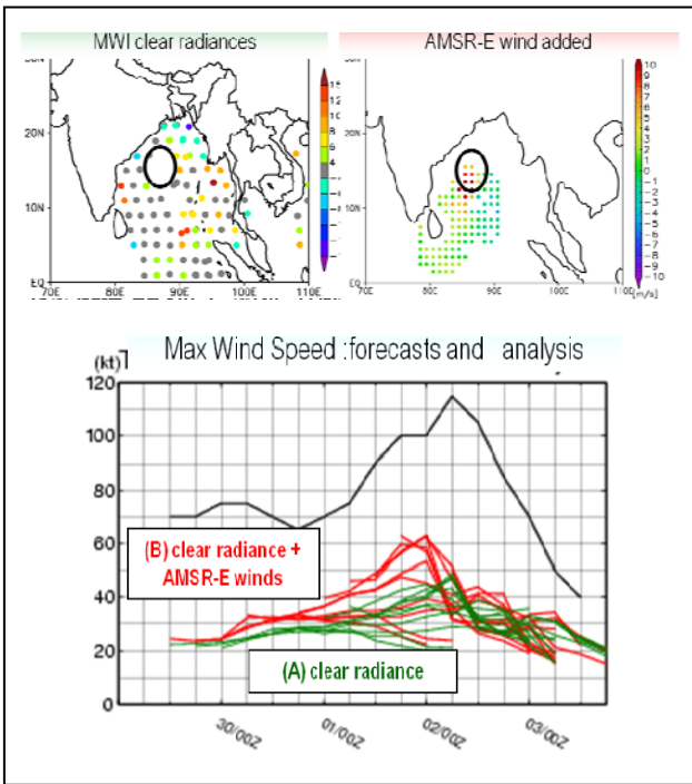
Figure 4. Example of improvement in maximum wind speed forecast by using AMSR-E all-weather wind speed for the case of Cyclone Nargis passing over the Indian Ocean in May 2008. Upper-left and -right panels show microwave radiances under clear sky, which is usually used for forecasting, and AMSR-E all-weather wind speed. Lower panel shows analysis (black), forecast just using clear microwave radiance (green), and forecast using AMSR-E winds in addition (Kazumori, 2009).
