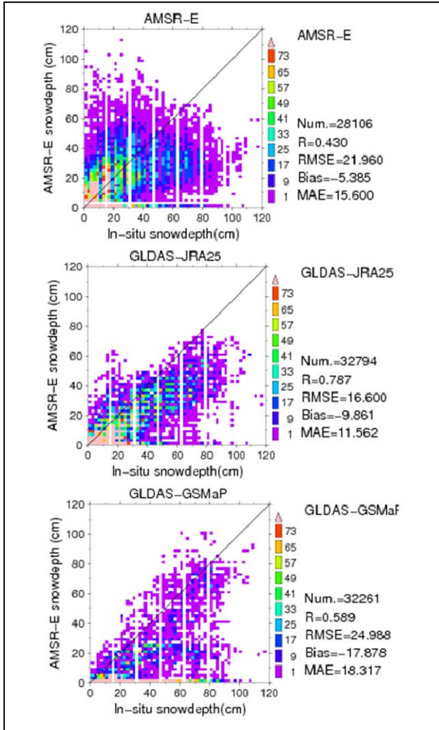
Figure 2. Upper: Daily mean comparison of in-situ measurement of snow depth and that retrieved from AMSR-E from 2003 to 2004. Middle: Same as upper panel but for snow depth calculated from Iso-MATSIRO using JRA-25 as input (GLDAS-JRA25). Bottom: Same as middle panel but replaced model rainfall to satellite-based rainfall (GLDAS-GSMaP).
